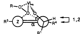
preferred transition state for m -CPBA epoxidations
