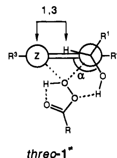
preferred transition state for m -CPBA epoxidations
